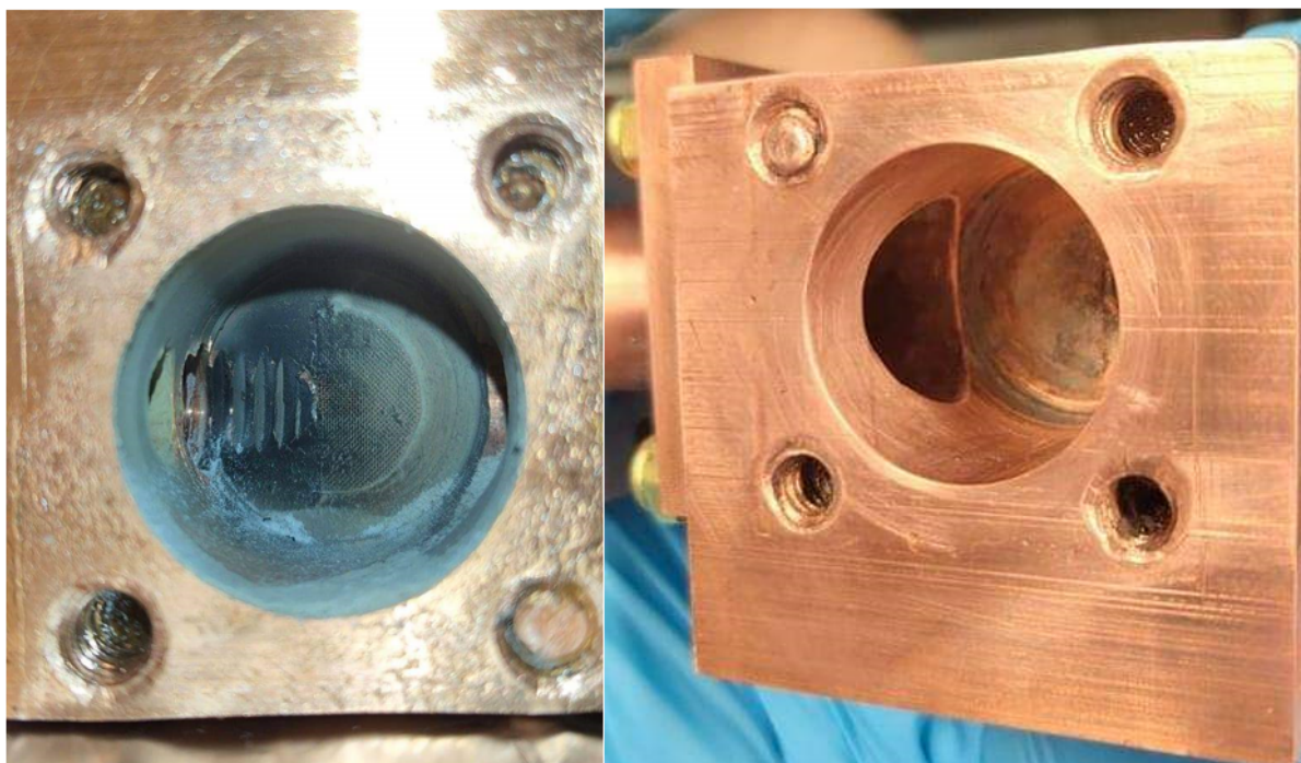
Figure 3.8: On the left, I show images of a cell after weeks of ablation. The powder seen at the bottom of the cell is debris blasted off the sample by the focused ablation laser. On the right, I show the cell after we sanded it and destroyed the beam.
