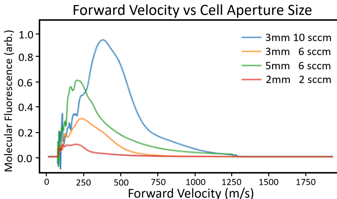
Figure 4.21: I show the effect of the cell aperture size for different He flow regimes. We seek to optimize the molecular yield at low velocity. Therefore, we chose to operate the cell with a 5mm aperture while flowing 4sccm of He.
