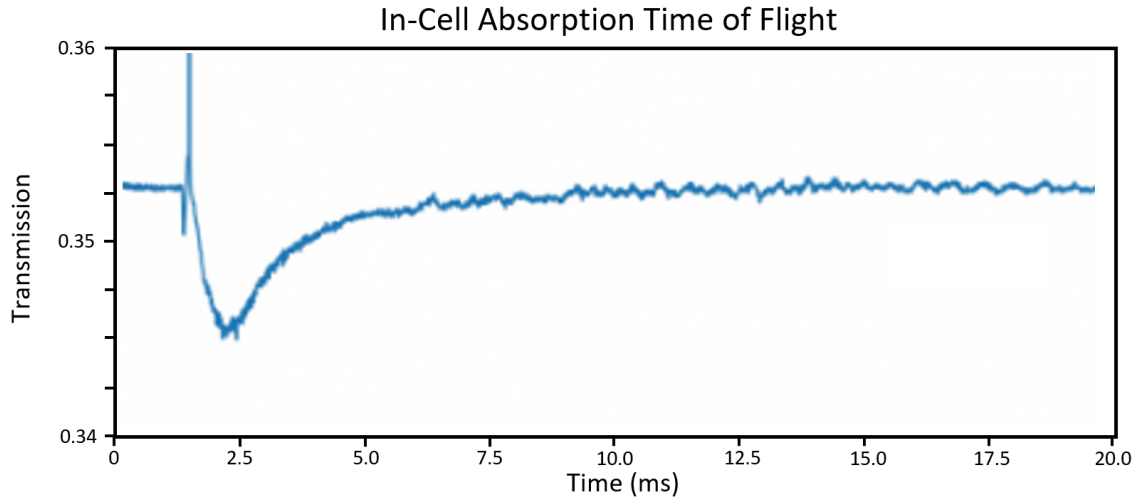
Figure 3.21: InGaAs fast photo-diode (top). [165] An example time of flight in-cell absorption trace recorded with a InGaAs fast photo-diode.
