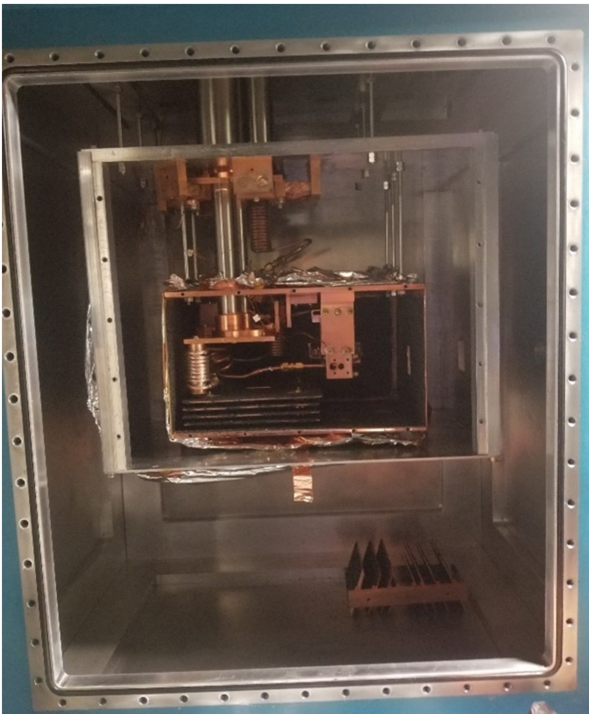
Figure 3.4: I show all the layers of the cryostat after we opened the system for cell maintenance. The room temperature shield can be seen on the outer edge along with the rubber gasket which provides the air-tight seal. A bank of cryogenic charcoal sorb fins can be seen resting on the base of the room temperature shield. Within , the aluminum 40K shield can be seen encasing the copper 4K region. Within, the 4K region one may observe the 4K PTR head, the ablation cell, the helium buffer gas bobbins, and additional charcoal sorbs.
