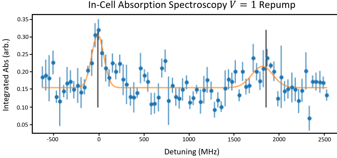
Figure 4.10: A 3GHz wide in-cell absorption spectrum in which both spin rotation states of the X^2\Sigma^+(V=1) \rightarrow B^2\Sigma^+(V=0) repumping transition can be seen. Two Gaussians have been fit to the resonances to guide the reader's eye and fit the center of each transition.
