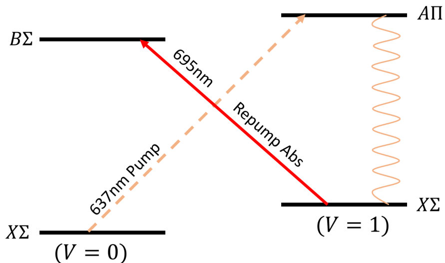
Figure 4.7: Shown in orange, is the pumping scheme used to populate the V=1 ground state. Absorption spectra were performed on the off-diagonal transition (shown in red) to return molecules in the V=1 X^2\Sigma^+ to the V=0 band through the intermediary B^2\Sigma^+ .
