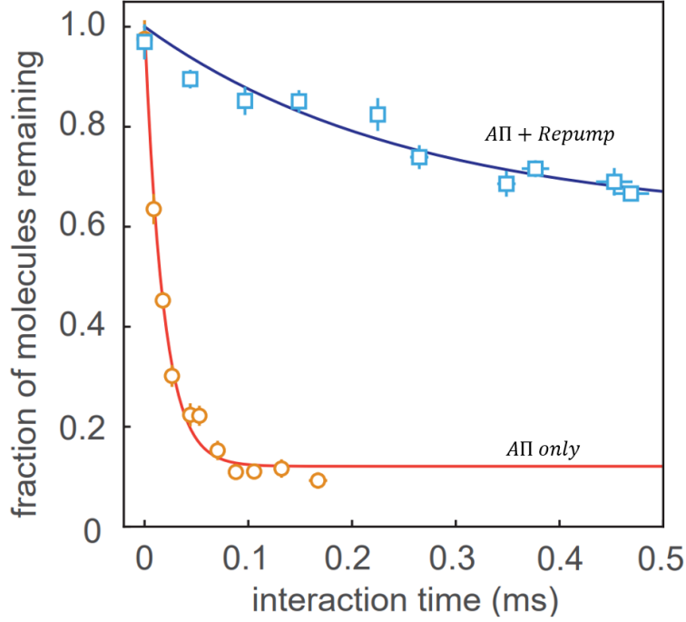
Figure 5.21: I show the depletion of the ground state when driving the X^2\Sigma^+(V=0) \rightarrow A^2\Pi alone (orange trace). Depletion of the ground state when driving the X^2\Sigma^+(V=0) \rightarrow A^2\Pi , while simultaneously applying the X^2\Sigma^+(V=1) \rightarrow B^2\Sigma^+(V=0) repumping laser (blue trace). The decay seen in the blue plot is due to the decay to the V=2 vibrational band.
