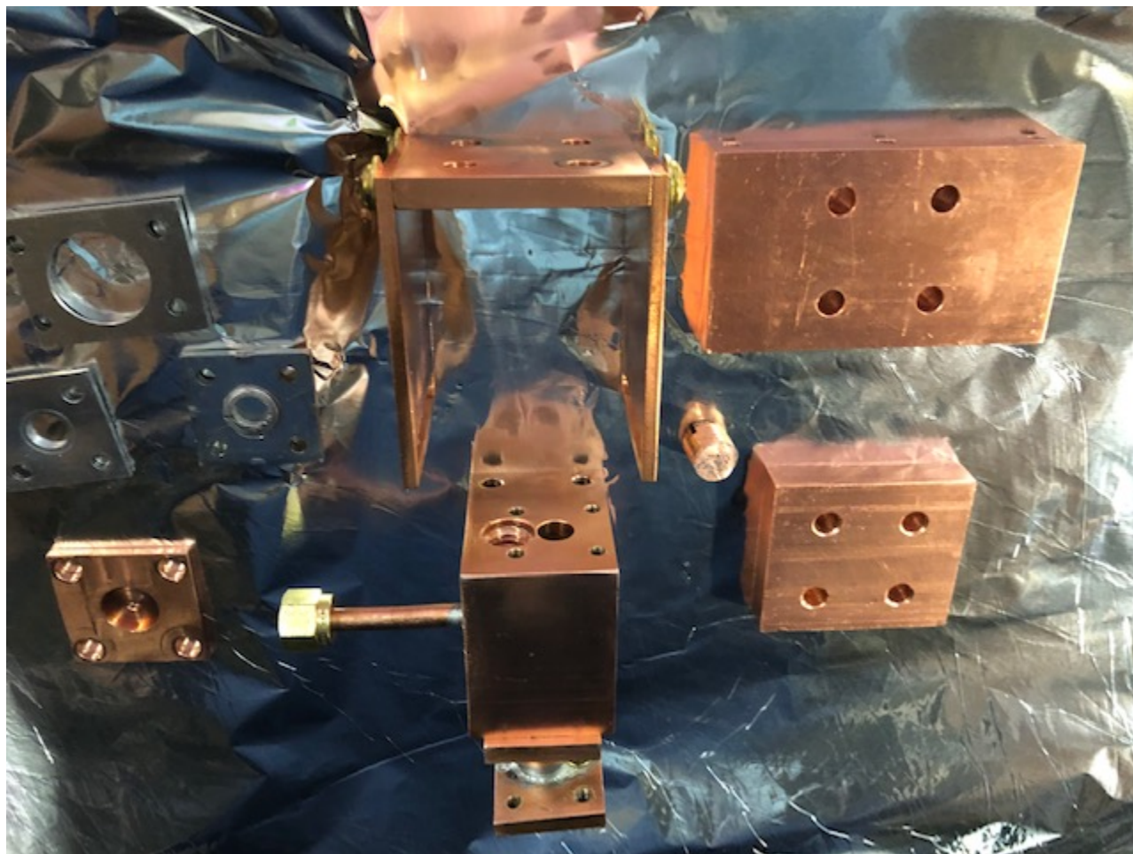
Figure 3.6: I show the components of the cell assembly after it was taken out of the cryostat. I show the cell, the cell windows, the cell aperture, the sample holder, and the thermal coupling plates.
