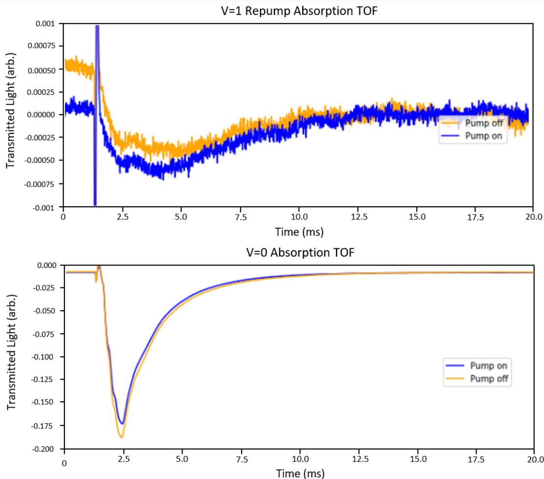
Figure 4.9: This figure shows the effect on the repump absorption time of flight by adding the V=1 pumping laser. The top plot shows the time of flight enhancement as detected through absorption on the X^2\Sigma^+ \rightarrow B^2\Sigma^+ . The bottom plot shows the time of flight depletion of the V = 0 ground state when the V = 1 pump is turned on. The orange plots corresponds to the absorption signal without the V = 1 pump, while the blue trace shows the time of flight when the V = 1 pump is turned on. These are single shot absorption traces.
