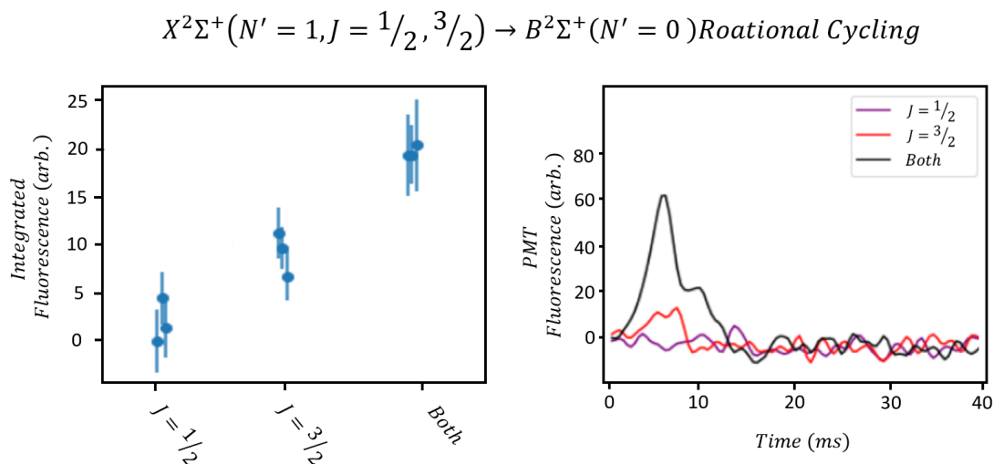
Figure 5.17: On the left, I show the molecular fluorescence from driving the J = 1/2 or J = 3/2 branch of the X^2\Sigma^+ \rightarrow B^2\Sigma^+ transition. Then, I show the enhanced fluorescence when both spin-rotation components are addressed, indicating that molecules were being transferred between the spin-rotation states, rather than being pumped into a dark state. On the right, I show the time of flight data corresponding to the integrated signals shown on the left.
