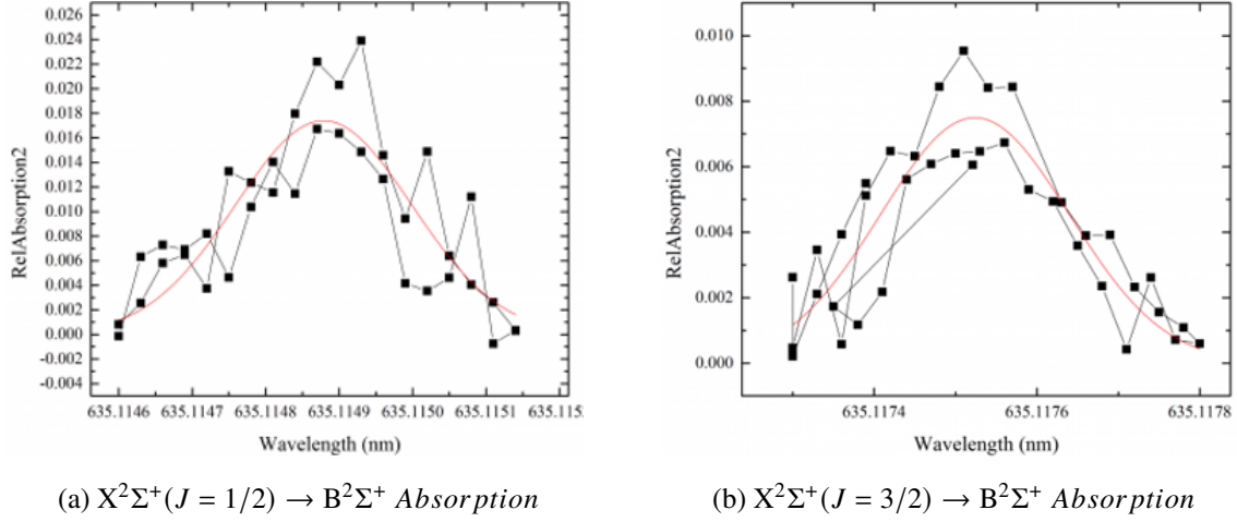
Figure 4.4: In-cell absorption spectra of the J=1/2 and J=3/2 branches of the X^2\Sigma^+ \rightarrow B^2\Sigma^+ transition.
